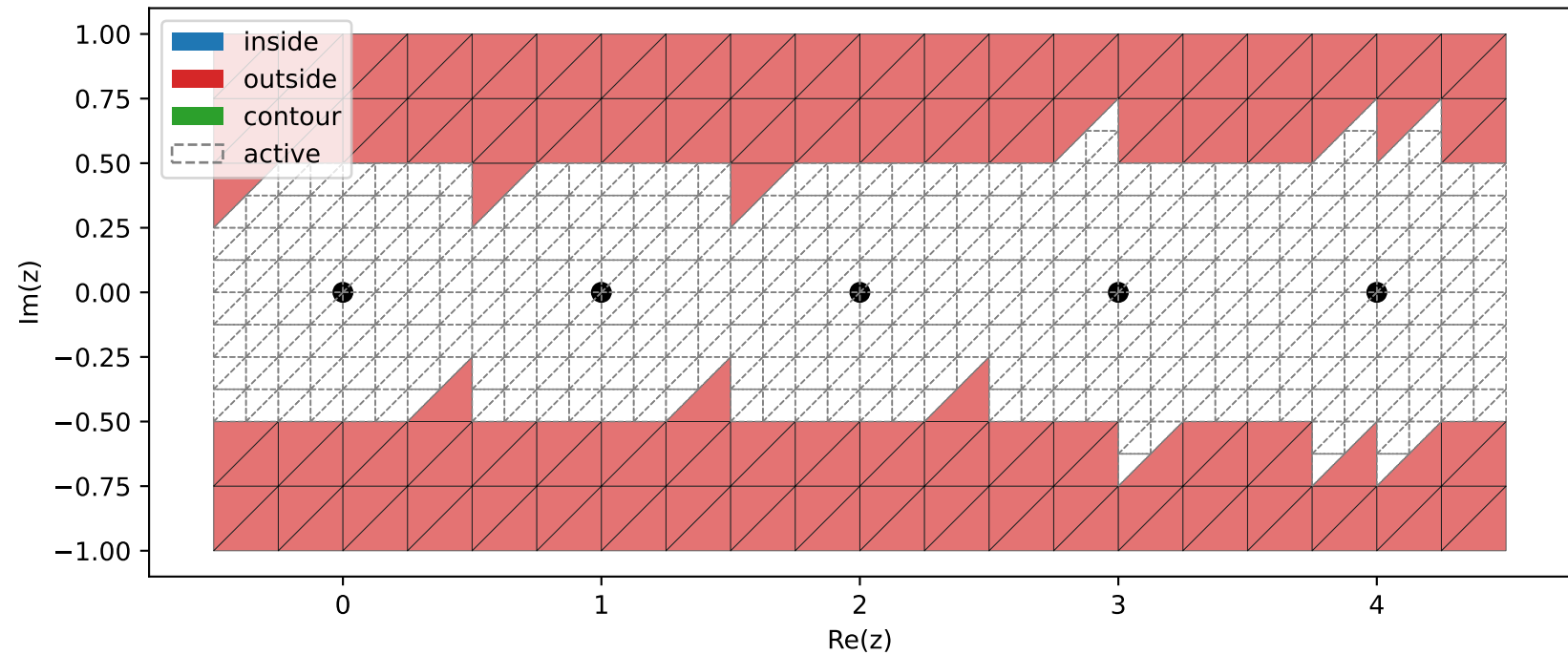
Outer-loop classification: sweep 0
